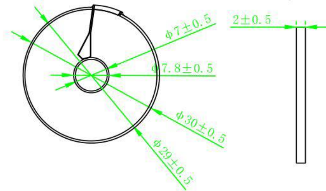
Antifreeze plate
