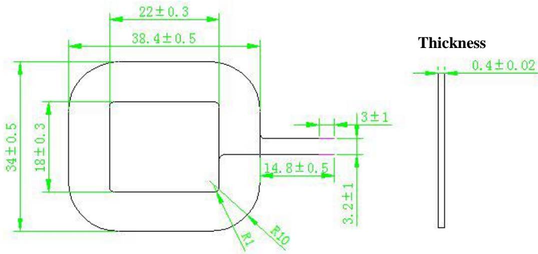
Coil
