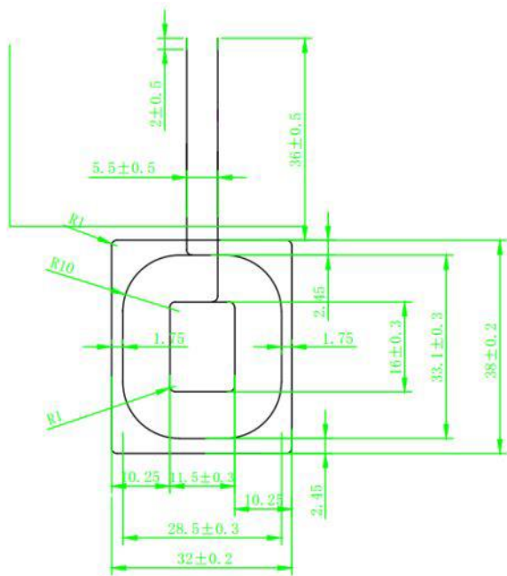
Coil
