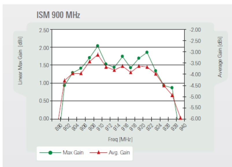
3D Max/Avg. Gain
