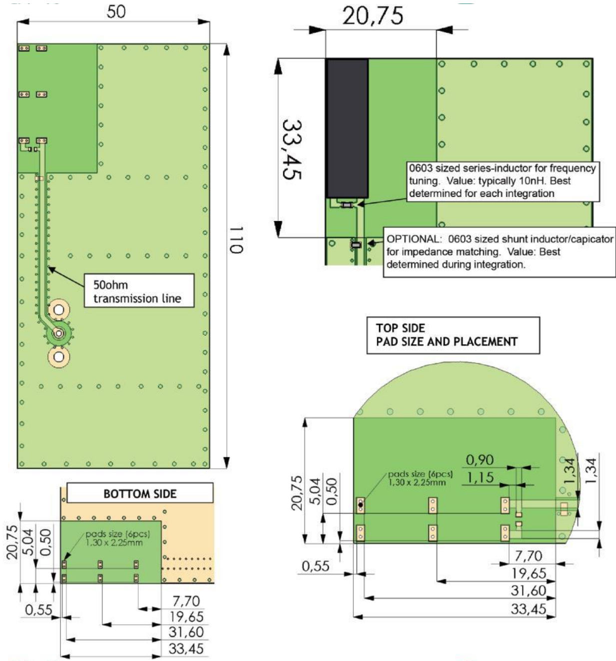
CW3544A- Antenna positioned vertically on PWB corner
